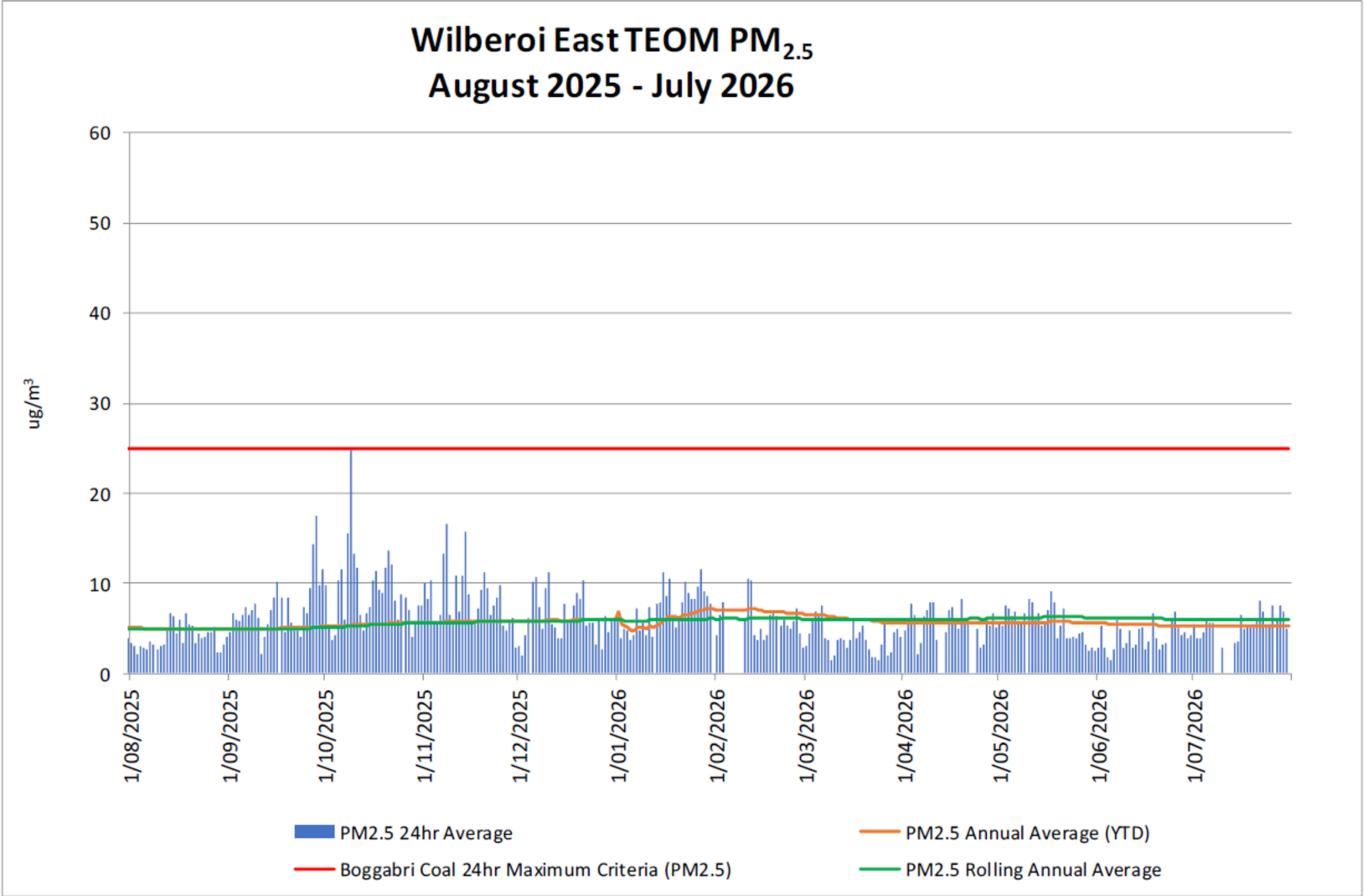
Figure 7: Wilberoi East PM 2.5 previous 12-month 24hr averages and annual YTD average
