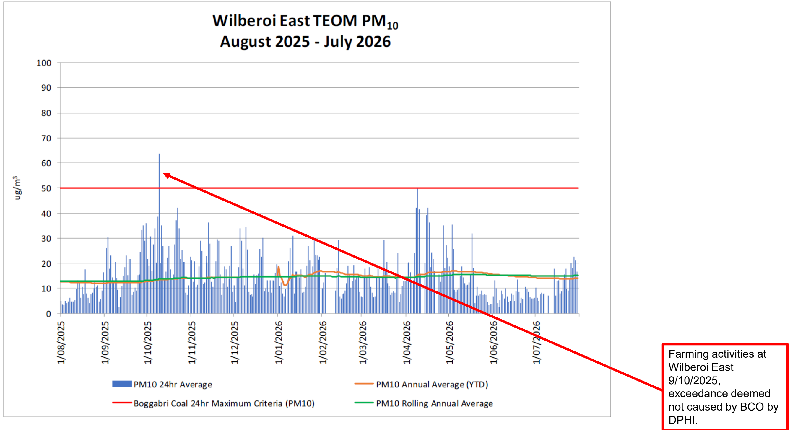
Figure 5: Wilberoi East PM 10 previous 12-month 24hr averages and annual YTD average
