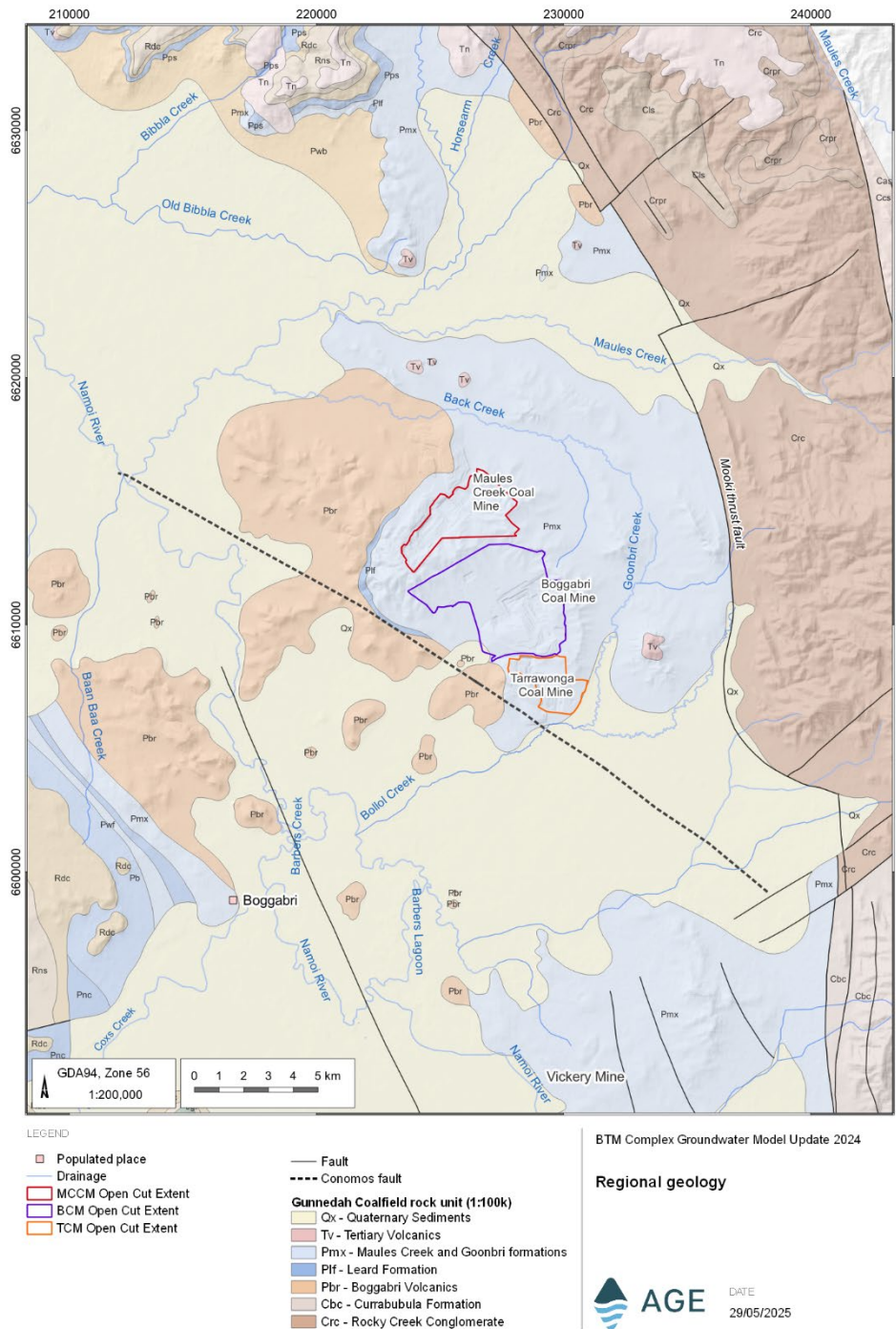
Figure 3.2 – Regional Geology
