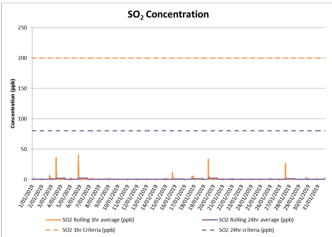
Figure 3 SO 2 Concentrations – January 2019
