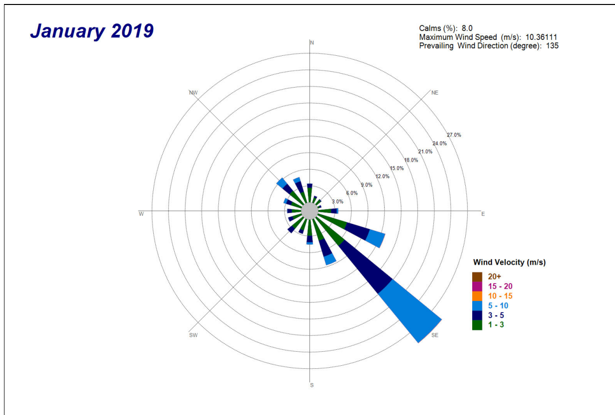
Figure 4 MCC January 2019 Meteorology Data
