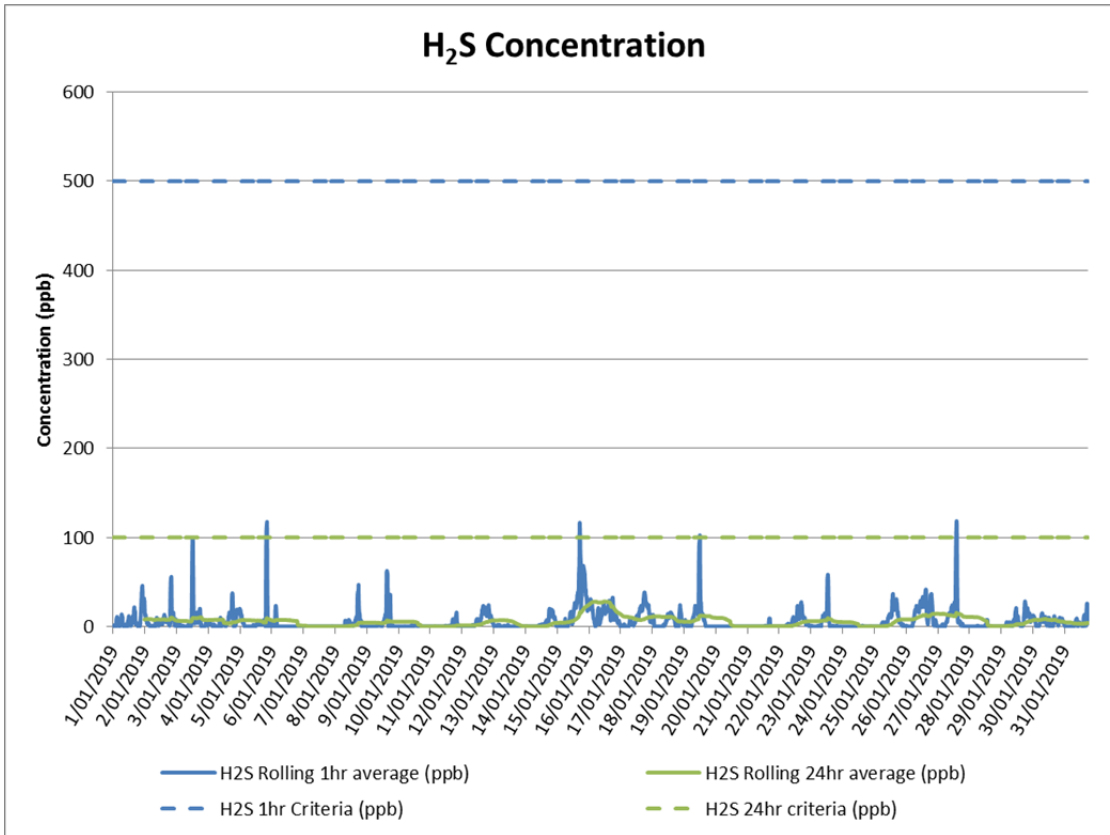
Figure 2 H 2 S Concentrations – January 2019
